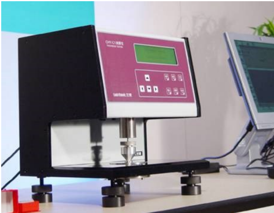
fig.1. Labthink CHY-C1
